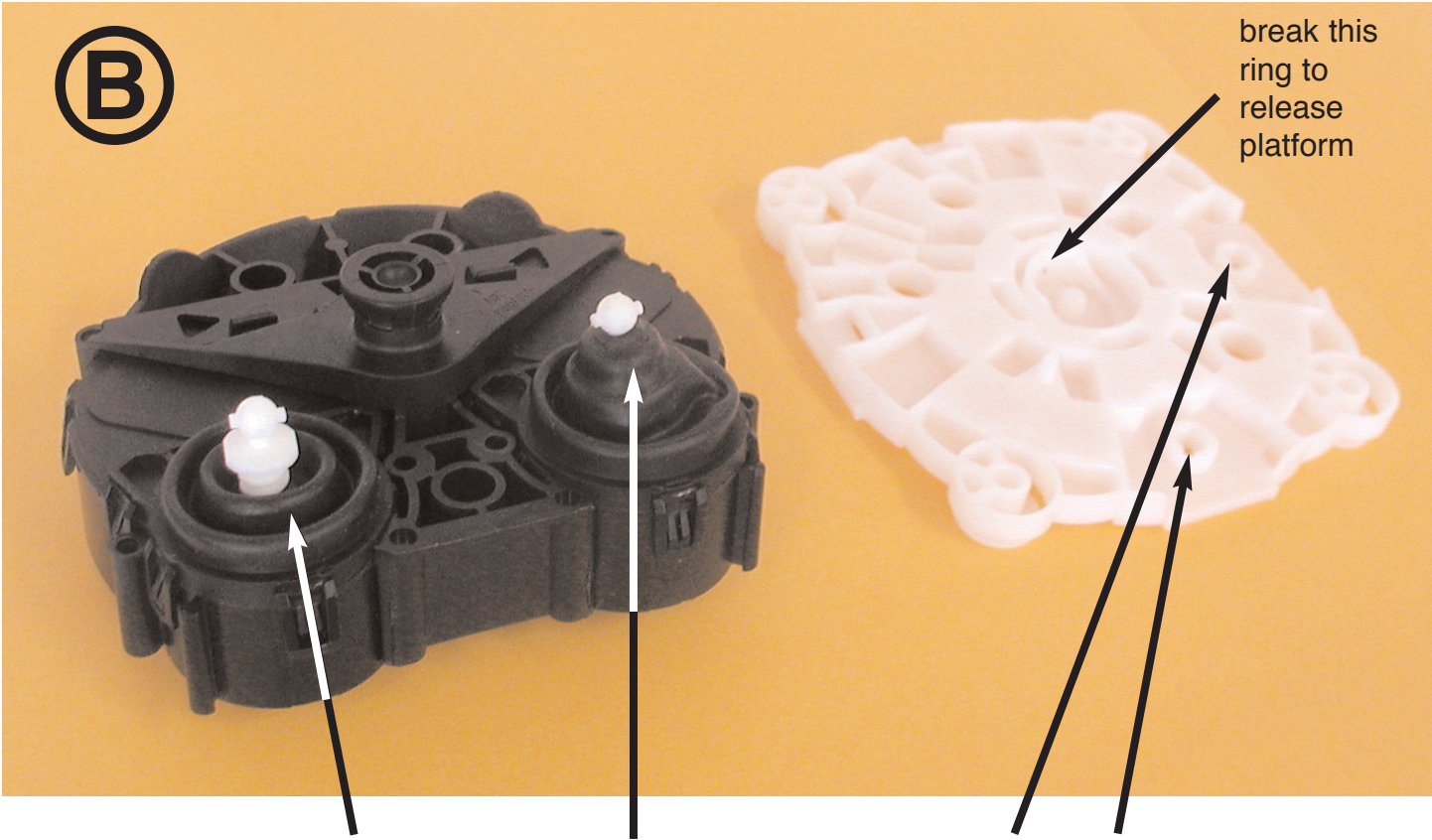
Keyed balljoints. Turn to remove from holes in platform.
