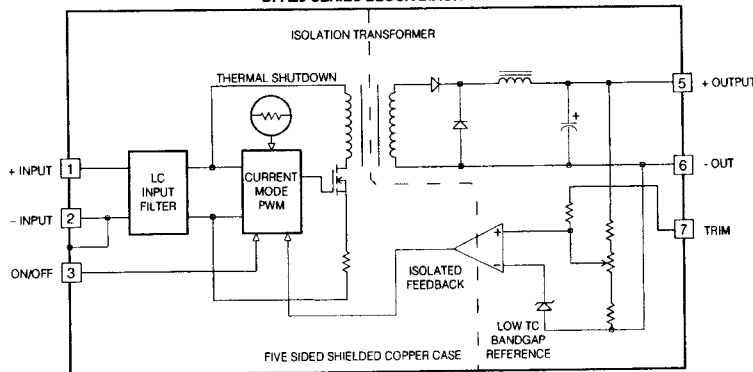
DFA20 SERIES BLOCK DIAGRAM
