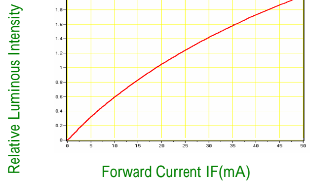
Relative Luminous Intensity-IF (Ta=25 )
