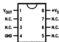
SO-8 Small Outline Molded Package
