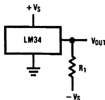
FIGURE 2. Full-Range Fahrenheit Temperature Sensor
