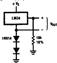
Temperature Sensor, Single Supply, -50° to +300°F
