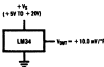
FIGURE 1. Basic Fahrenheit Temperature Sensor ( +5^\circ to +300^\circ\text{F} )
