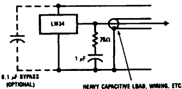
FIGURE 4. LM34 with R-C Damper
