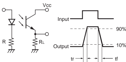
■ Response Time Measuring Circuit
