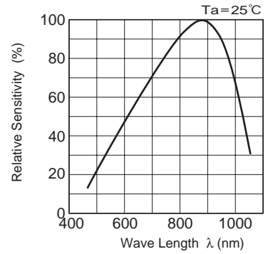
■ Spectral Sensitivity Characteristics
