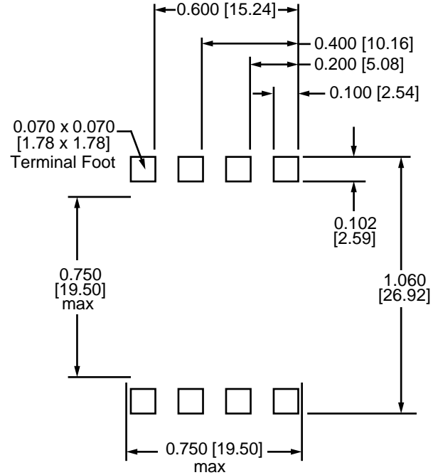
Suggested PCB Pad Layout
