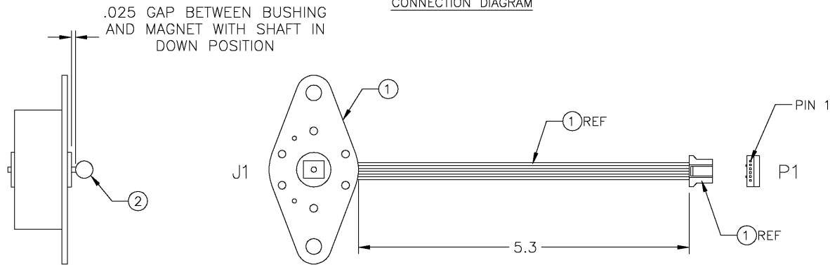
CONNECTION DIAGRAM
