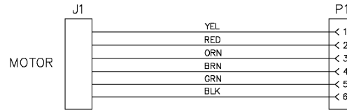
CONNECTION DIAGRAM
